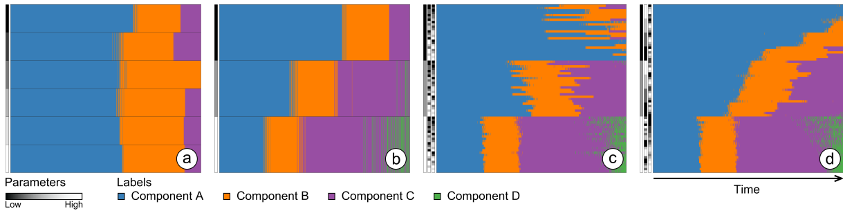
Figure 2: This figure shows a time series derived from a simulation model with three parameters describing bio-chemical reactions [MRU11]. Different segments are distinguished by color and each horizontal line represents a segmentation and labeling result. (a) Changing parameter 3 only slightly influences the results. (b) Different values for parameter 1 lead to quite different results. However, in both cases, all components are predominant for a certain period of time. This is not true for testing parameter combinations as shown in (c). Arranging the results by similarity (d) illustrates the complex influences of individual parameters.
