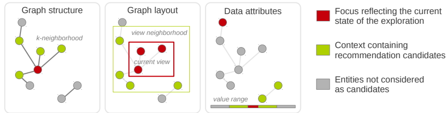
Fig. 3. Different definition of focus and context in terms of the graph structure, the graph layout, and the data attributes yield different candidates for recommendation.
