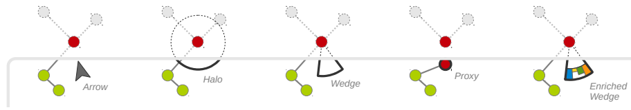
Fig. 4. Techniques for recommending navigation to off-screen nodes. Green nodes are on-screen, dashed elements are off-screen, and the red node is the recommend target.
