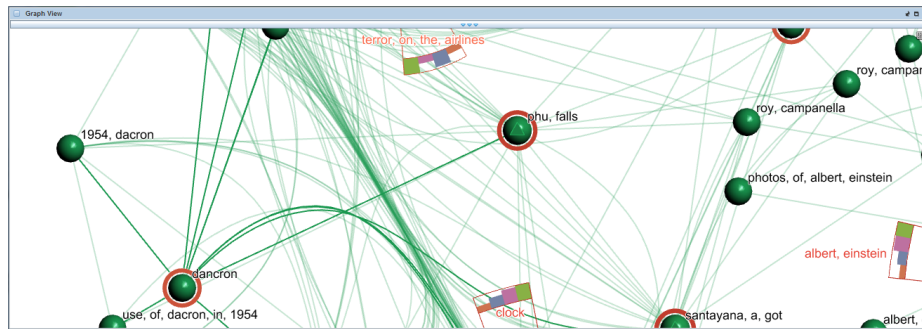
Fig. 6. Navigation recommendation in the proof-of-concept implementation. Red circles indicate on-screen targets worth investigating next. Enriched wedges indicate off-screen targets that might be of interest to the user as well.
